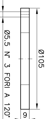
RONDELLA COD.202000102 Washer
