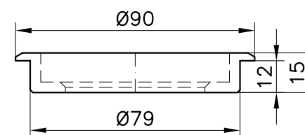
CORONA AD INCASSO COD.202000101 Crown embedded
