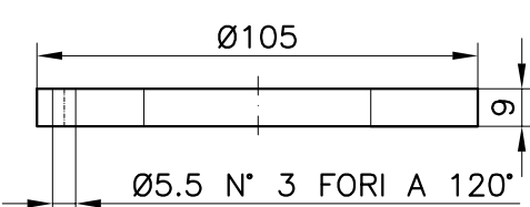
RONDELLA COD.202000102 Washer
