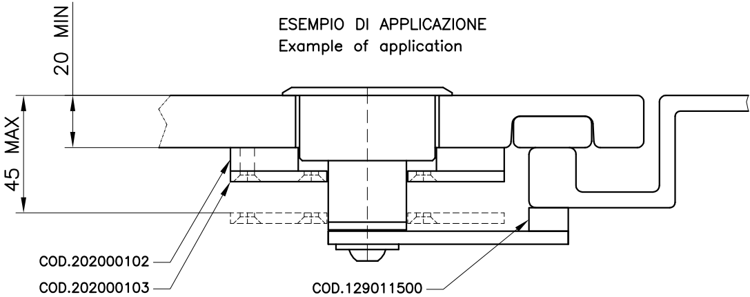
RONDELLA COD.202000102 Washer
