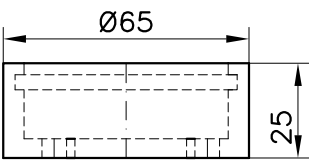
BOCCOLA COD.129011900 Bush
