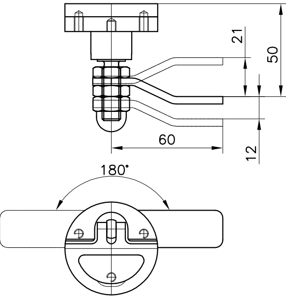
CHIUSURA COD.102100600 Closing
