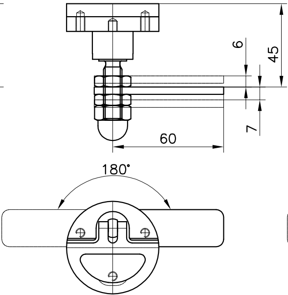
CHIUSURA COD.102100500 Closing
