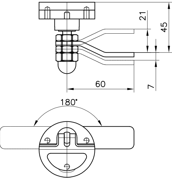
CHIUSURA COD.102100300 Closing
