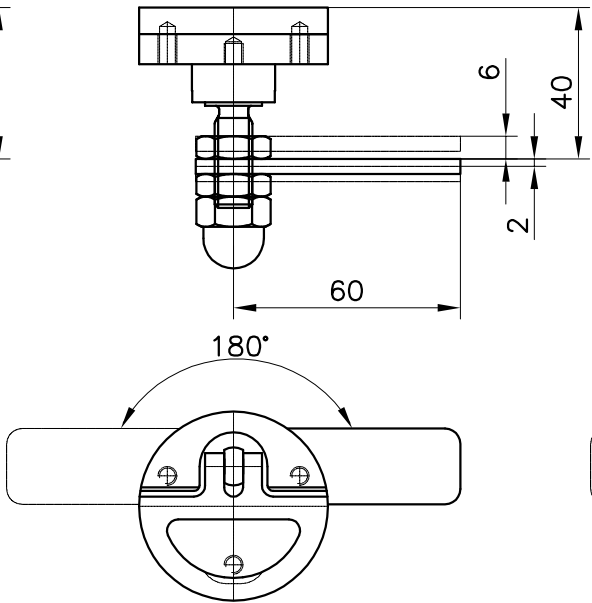
CHIUSURA COD.102100200 Closing
