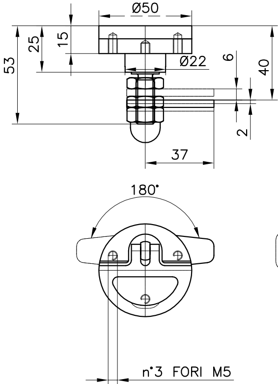
CHIUSURA COD.102100100 Closing
