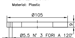
RONDELLA COD.202000102 Washer MATERIALE: PLASTICA Material: Plastic
